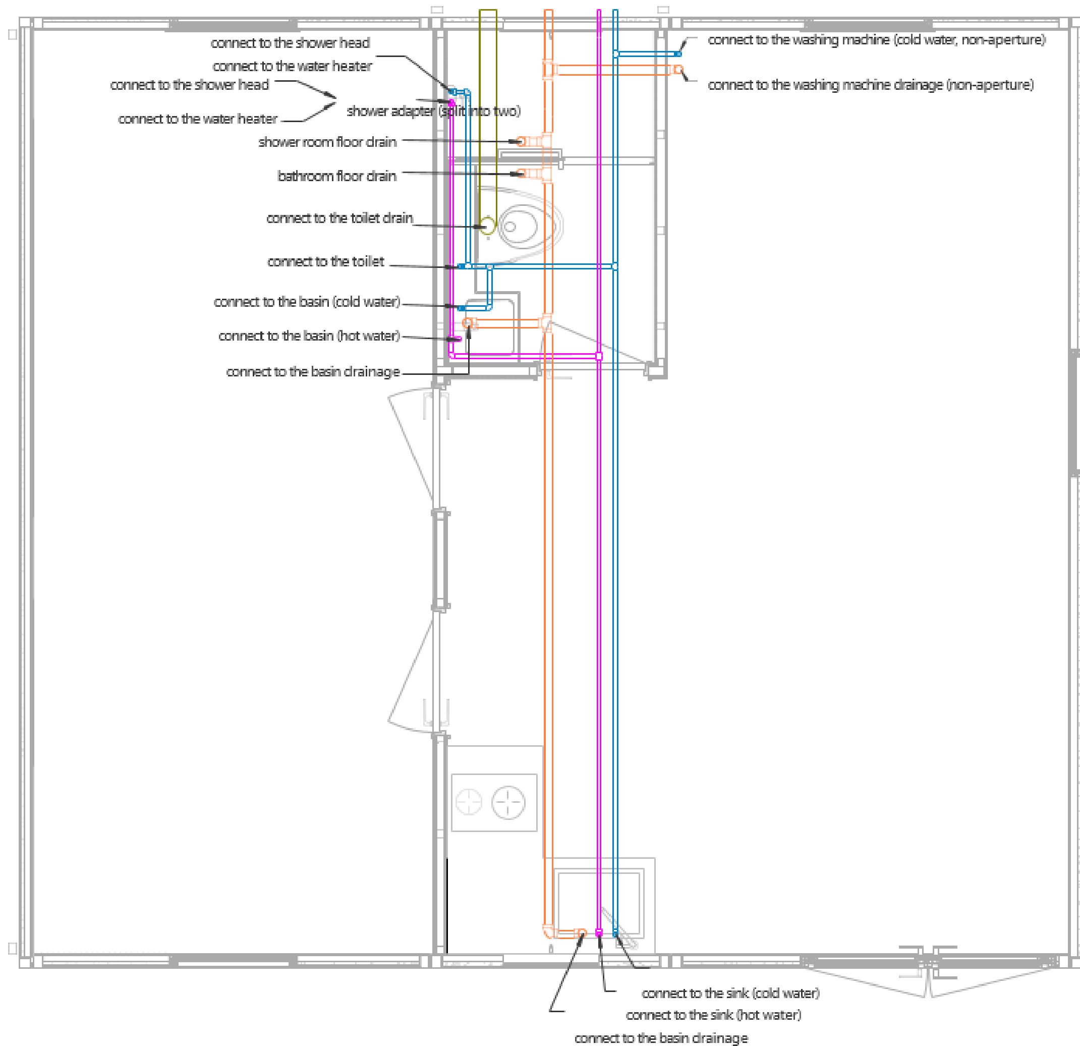
Water Supply and Drainage System Plan
