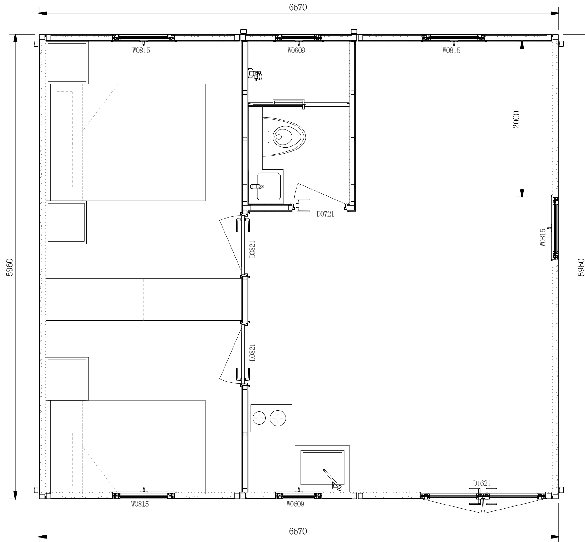
Layout Plan
