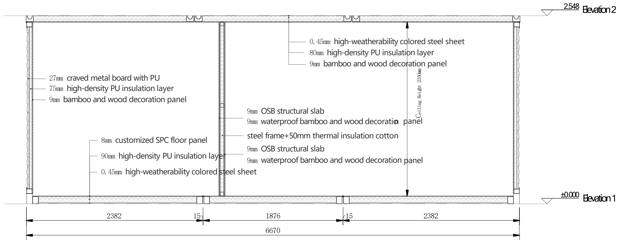
Section Plan
