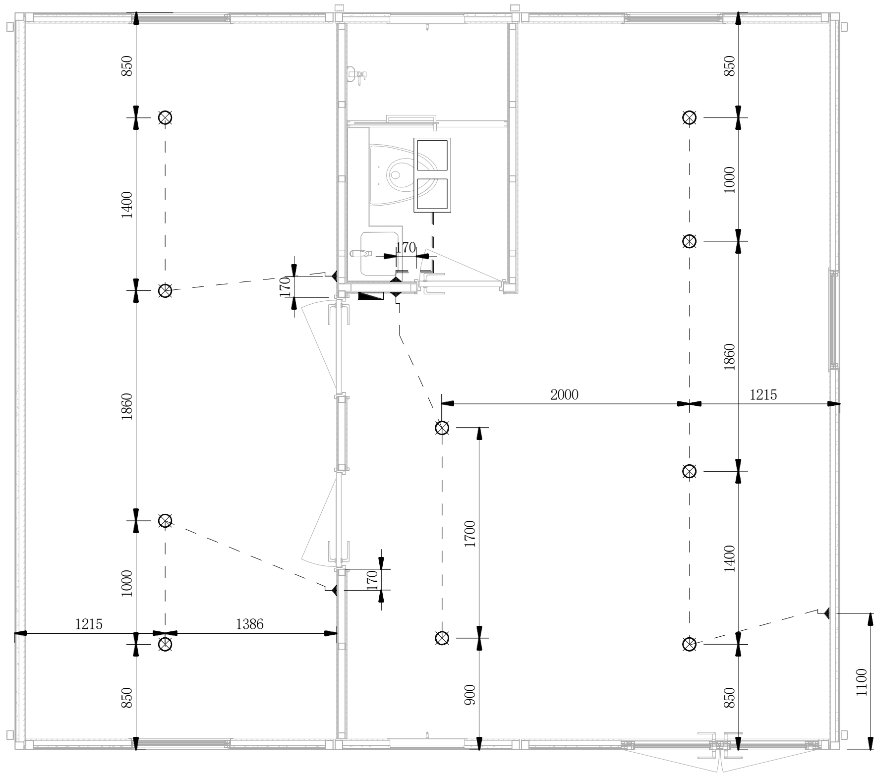
Lighting Plan
